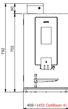
FRONT VIEW All dimensions in millimeters.
