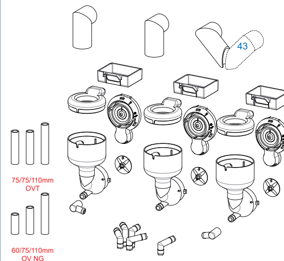
Hygiēneset 1003987 Optivend 33, 43, 33TS, 43TS NG
