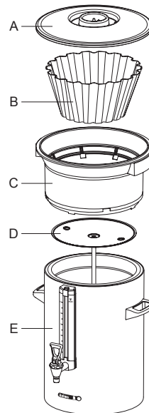
Container + accessories coffee Fig. 6
