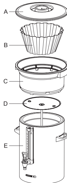
Container + accessories coffee Fig. 6
