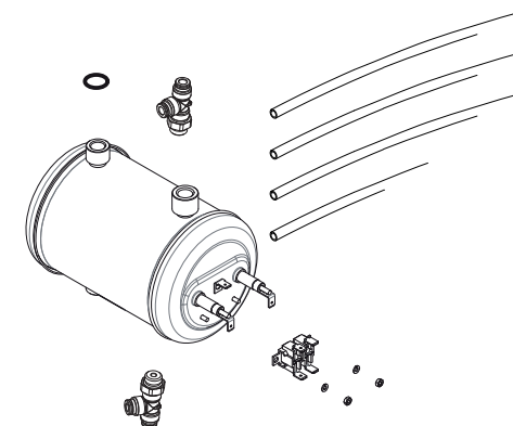
1011131* Boiler replacement kit OptiBean X
