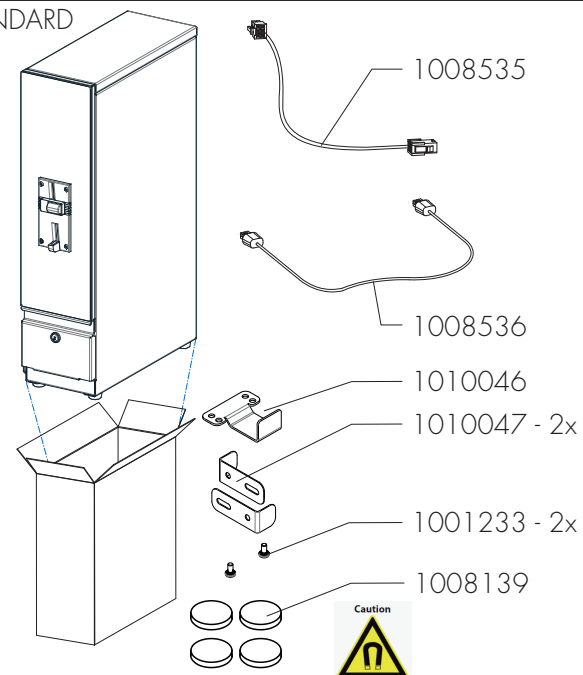
1010305 HOUSING FOR CASHLESS
