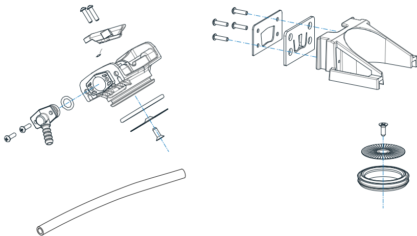
1011062* Replacement Kit Brewer X Press
